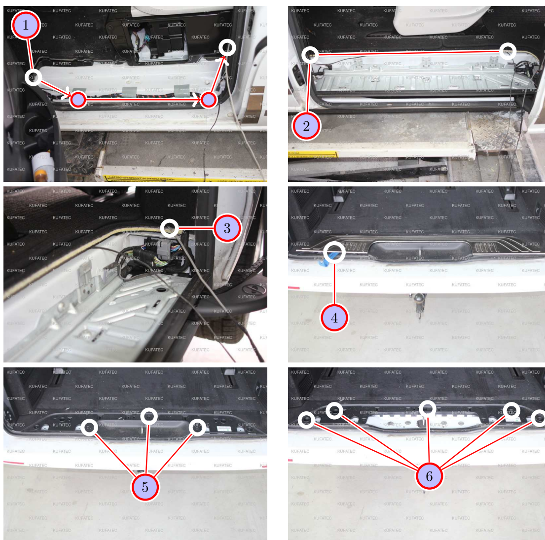
Figure 8: Routing cable sound generator - pictures
