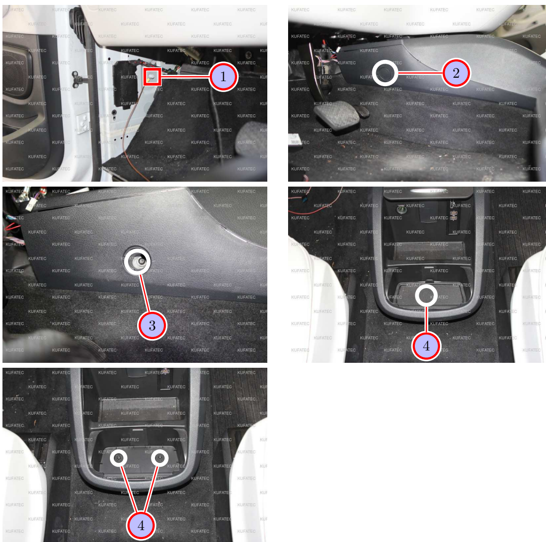
Figure 5: Connection ground / removing center console - pictures
