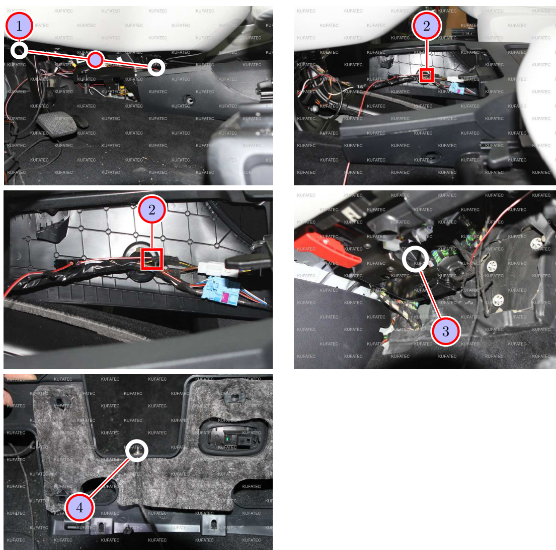
Figure 6: Connection ignition lead / control unit / module - pictures
