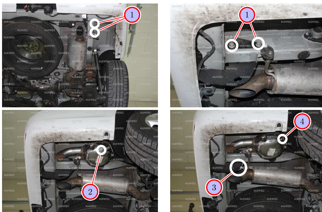
Figure 10: Installation sound generator - pictures
