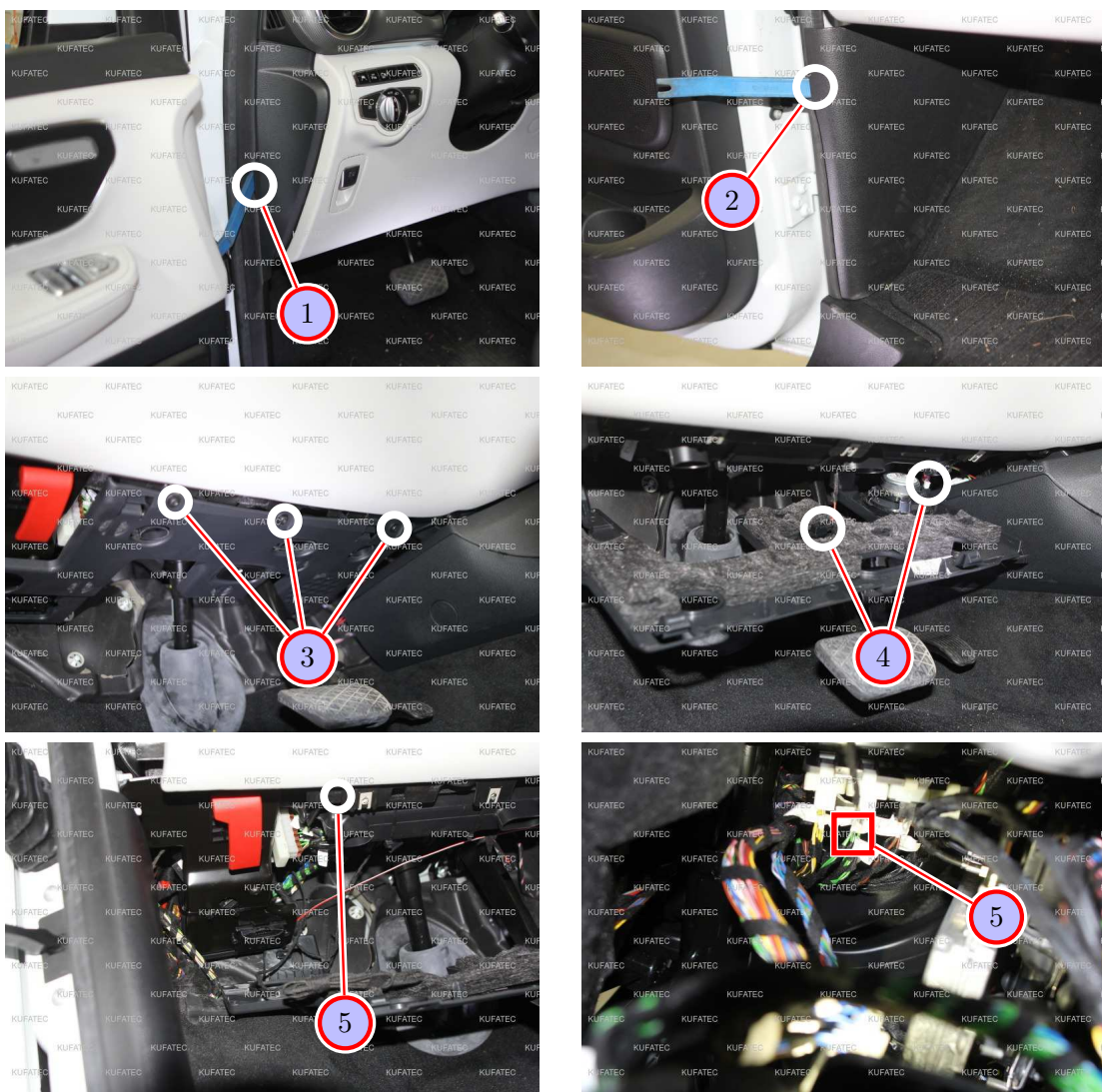
Figure 4: Connection CAN-High / CAN-Low - pictures
