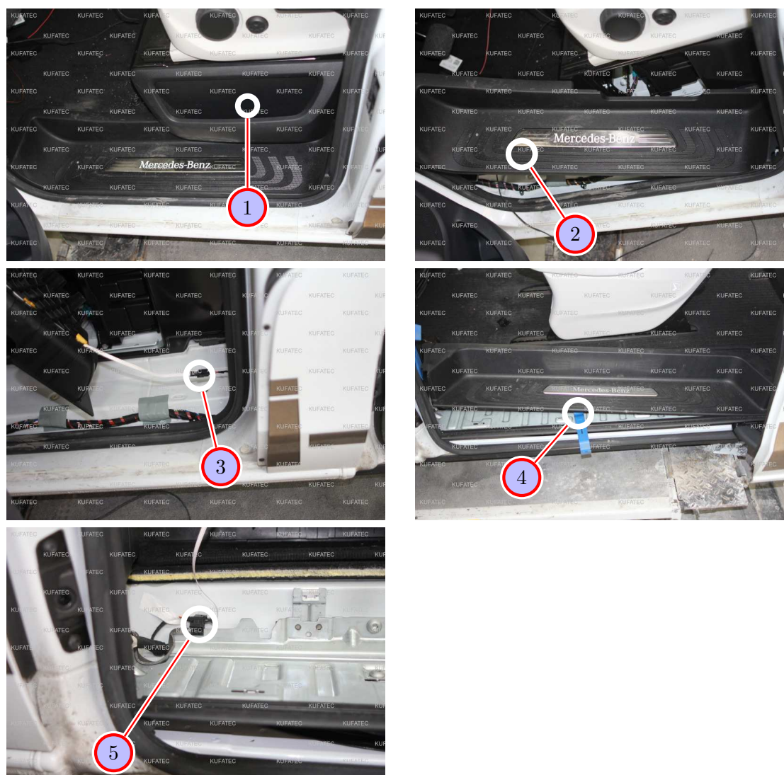
Figure 7: Removing sill trims front / rear - pictures
