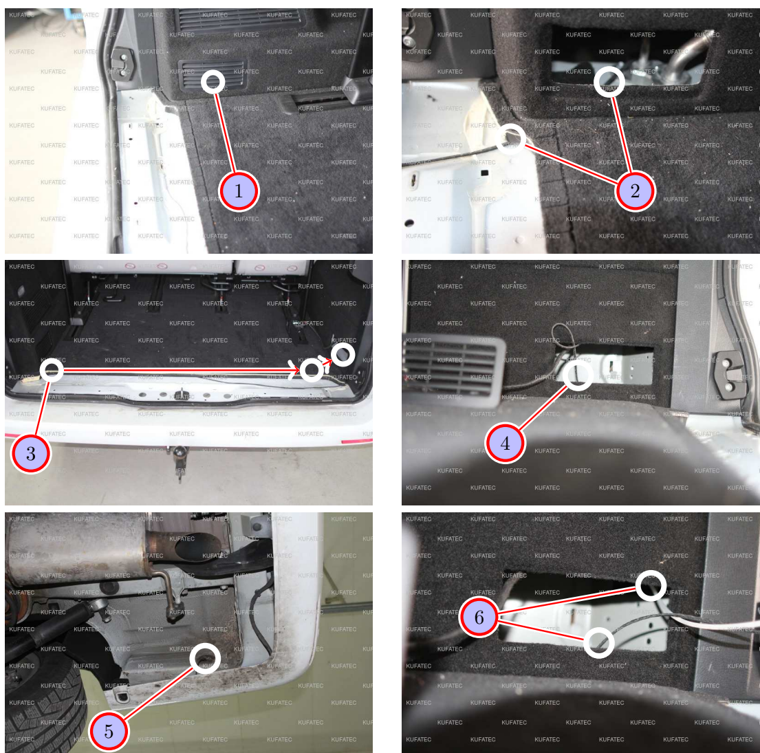
Figure 9: Routing cable sound generator to the underbody - pictures
